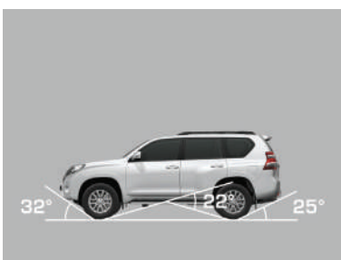
5-door | Approach, ramp breakover and departure
